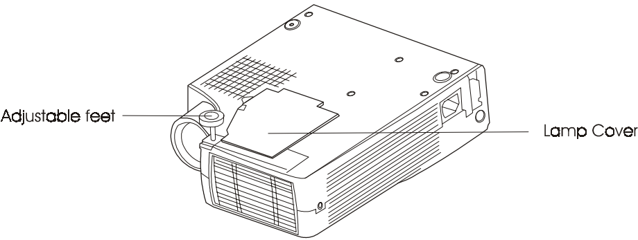
Figure 3 Bottom view
